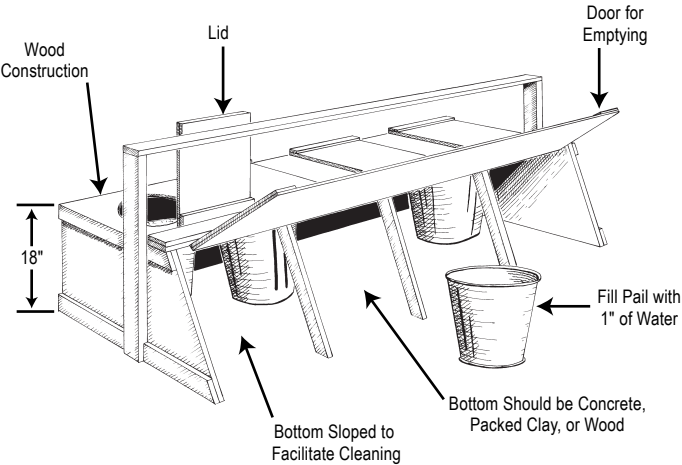
Figure 5-13: Pail Latrine
